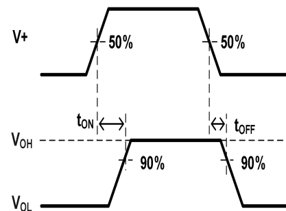
Fig.8-2. Turn-On ( t_{ON} ) and Turn-Off Time ( t_{OFF} )
