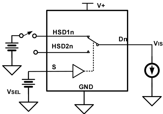
Fig.8-1. ON-State Resistance ( R_{ON} )
