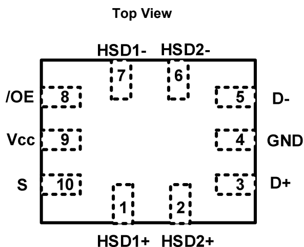
Fig.5-1.GT4222: QA (QFN1.4*1.8-10L) Package
