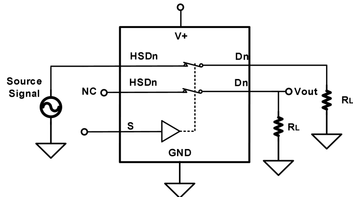
Fig.8-5. Channel-to-Channel Crosstalk
