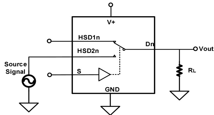
Fig.8-4. Off Isolation(OIRR)
