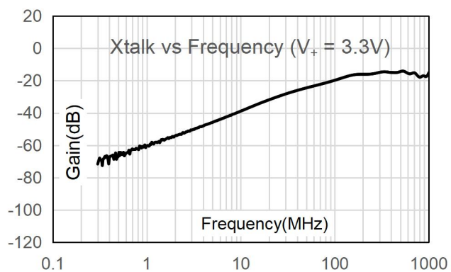
Fig.8-5. Xtalk vs Frequency at 3.3V V_+
