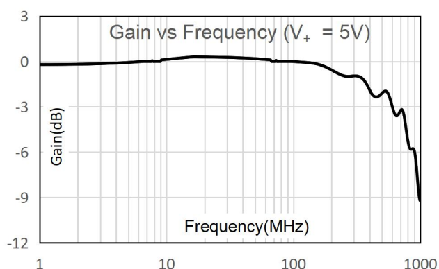
Fig.8-2. Bandwidth vs Frequency at 5V V_+
