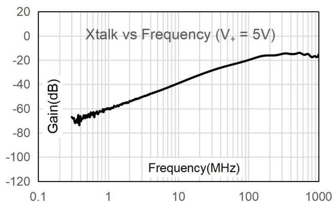
Fig.8-6. Xtalk vs Frequency at 5V V_+
