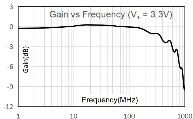
Fig.8-1. Bandwidth vs Frequency at 3.3V V_+
