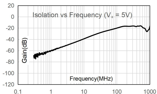
Fig.8-4. Isolation vs Frequency at 5V V_+
