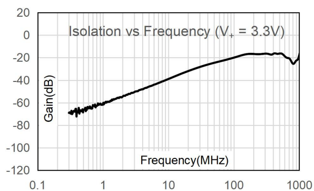
Fig.8-3. Isolation vs Frequency at 3.3V V_+
