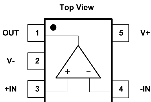
Fig.5-1. GT8521: S5(SOT23-5) Package
