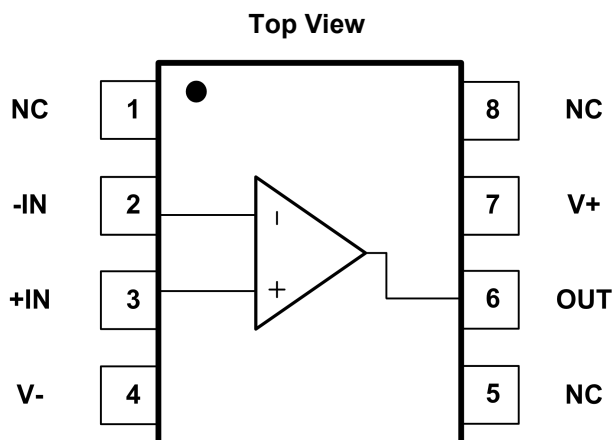
Fig.5-2. GT8521: P8(SOP8) Package
