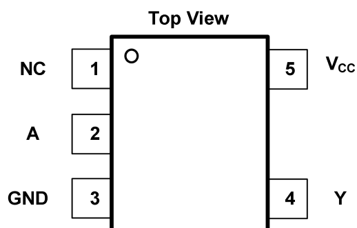
Fig.5-1. GT74LVC1G14: S5 (SOT23-5) Package
