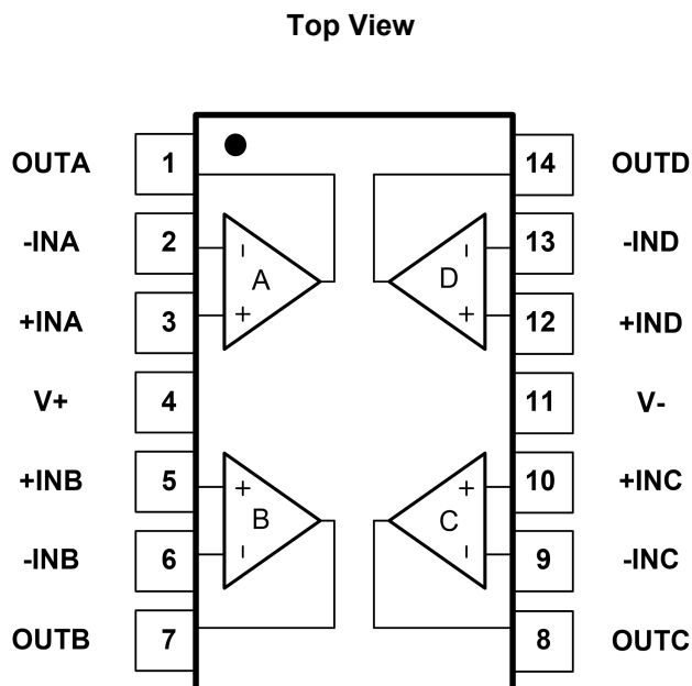
Fig.5-5. GT824: TD (TSSOP14) Package
