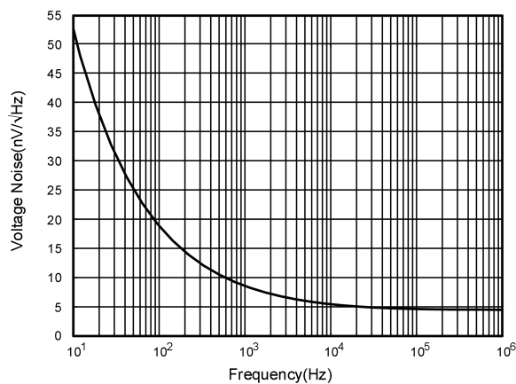
Fig.8-3. Voltage Noise vs Frequency
