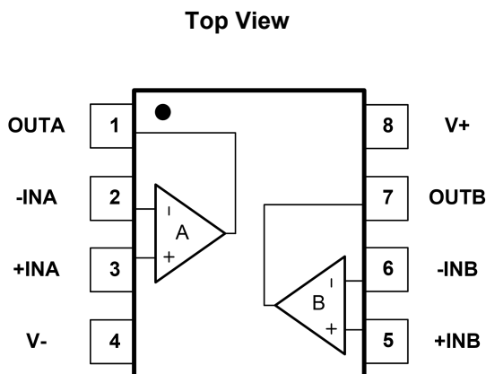
Fig.4-4.LMV358: M8(MSOP8) Package
