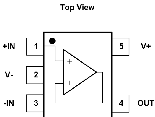
Fig.4-1. LMV321: C5 (SC70-5) Package LMV321: S5 (SOT23-5) Package
