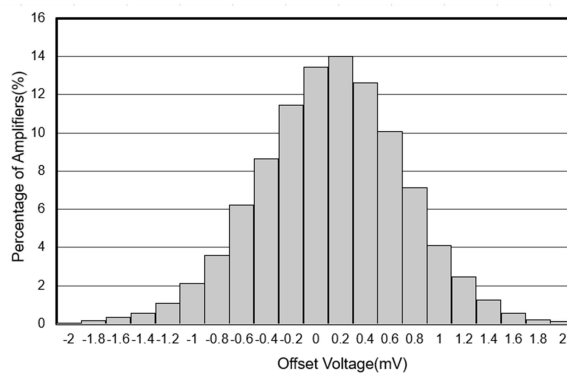
Fig.7-4. Offset Voltage Production Distribution (LMV321)
