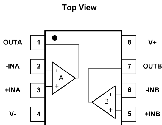
Fig.4-4.LMV358: M8(MSOP8) Package
