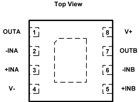
Fig. 4-5. LMV358: F8(DFN2x2-8) Package
